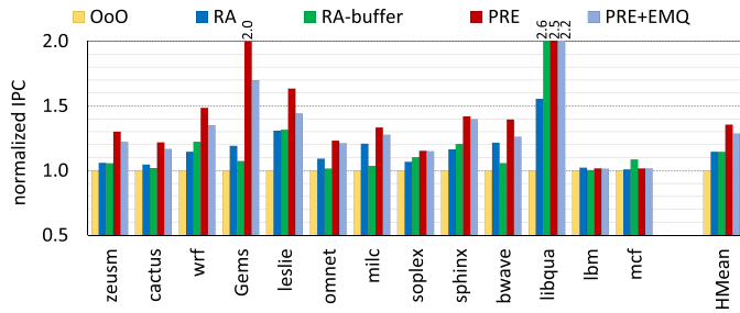
Fig. 2. Performance normalized to OoO.
